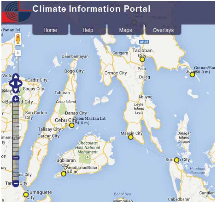
Figure 3. Climate stations close to Sugod (PH).
